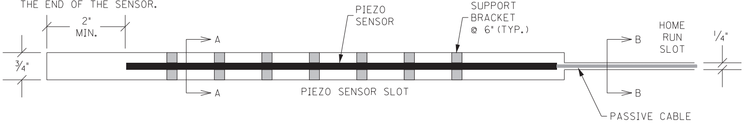
PLAN
