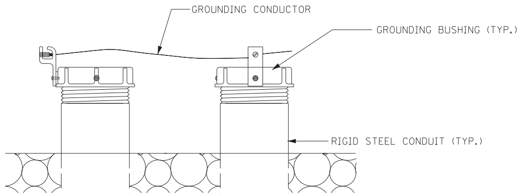
GROUNDING DETAIL
