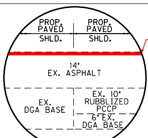
DETAIL "E" NOT TO SCALE
