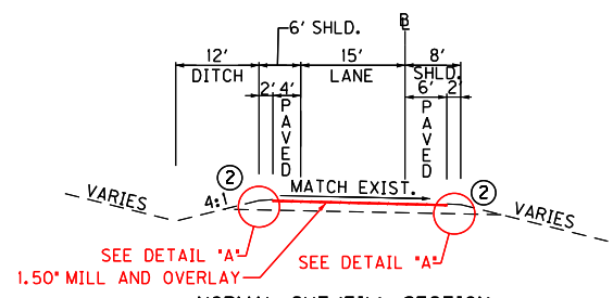
NORMAL CUT/FILL SECTION
