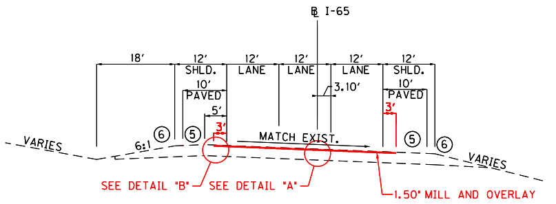
LEFT SUPERELEVATED SOUTHBOUND BIFURCATED CUT/FILL SECTION
