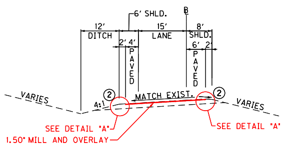
SUPERELEVATED LEFT CUT/FILL SECTION
