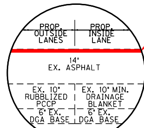
DETAIL "A" NOT TO SCALE
