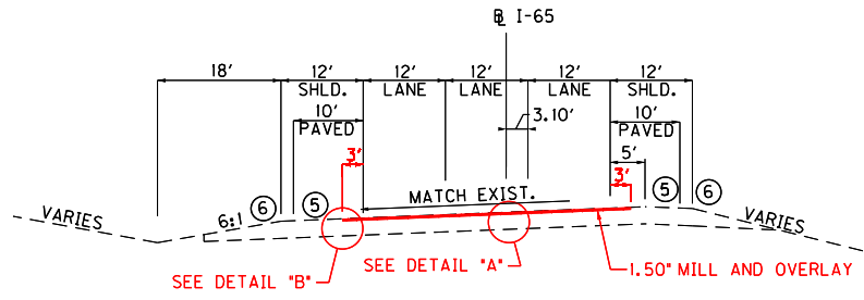
RIGHT SUPERELEVATED SOUTHBOUND BIFURCATED CUT/FILL SECTION
