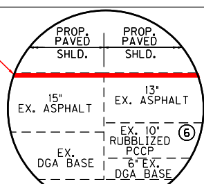
DETAIL "D" NOT TO SCALE
