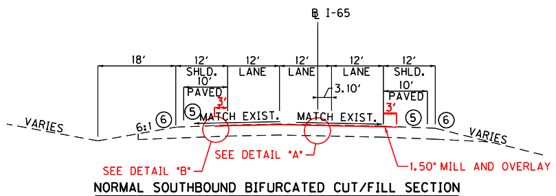
NORMAL SOUTHBOUND BIFURCATED CUT/FILL SECTION
