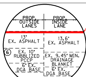
DETAIL "C" NOT TO SCALE
